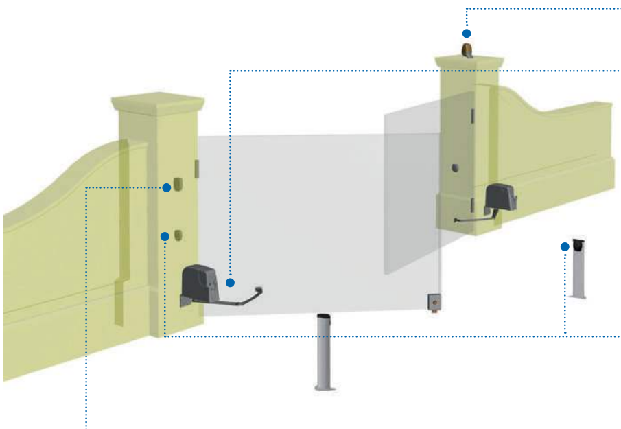
Photocellules LINEAR/XS
